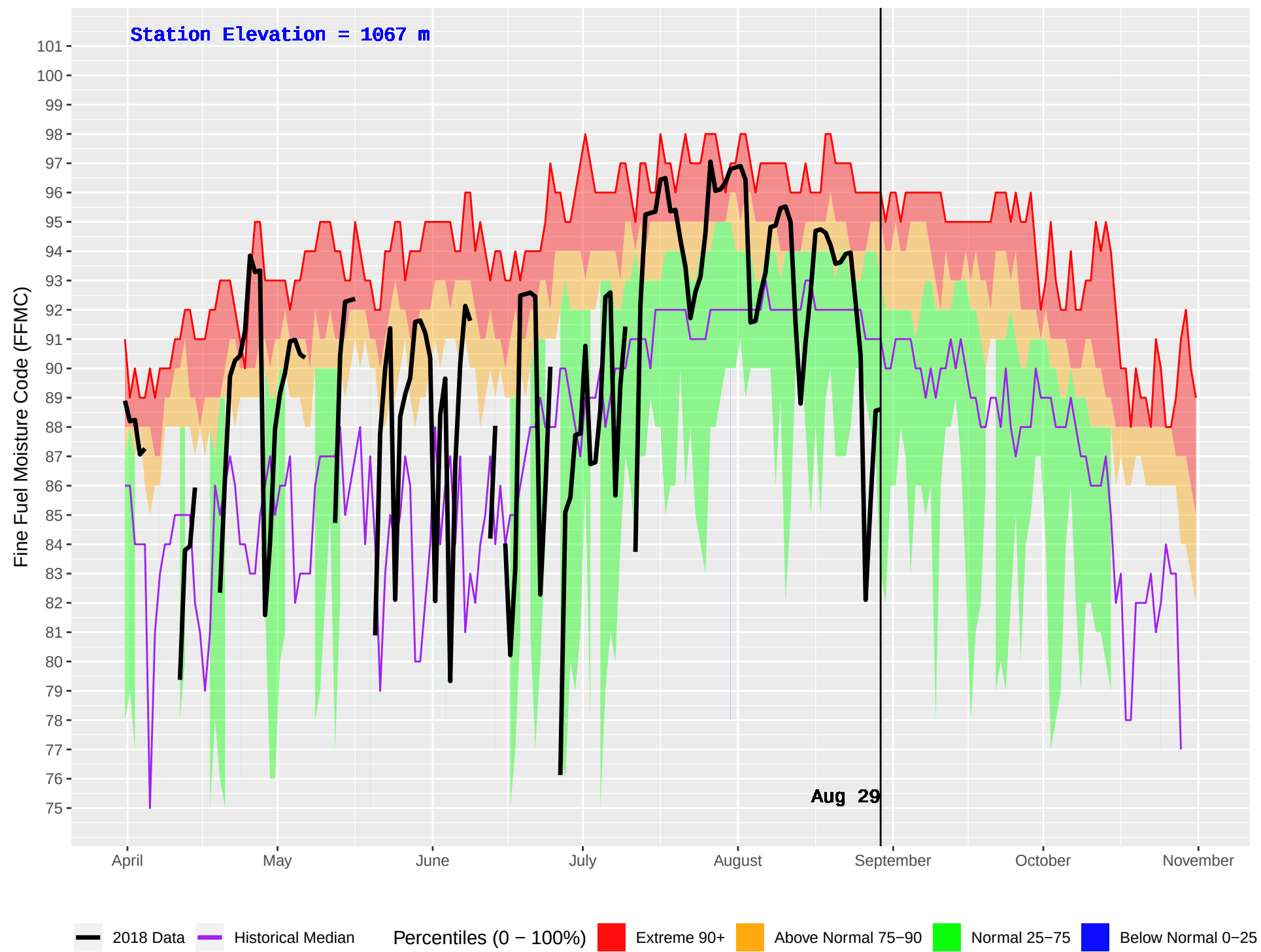
MCCUDDY (334) : Historical (1984–2016) and Current (2018) Daily Fine Fuel Moisture Code (FFMC)
