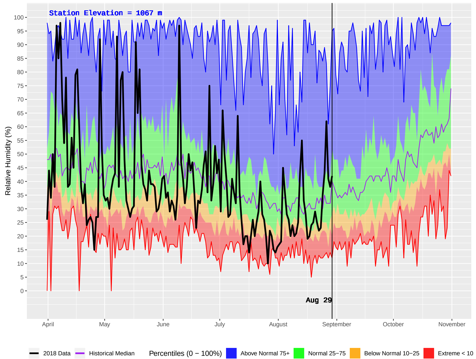
MCCUDDY (334) : Historical (1984–2016) and Current (2018) Daily Relative Humidity
