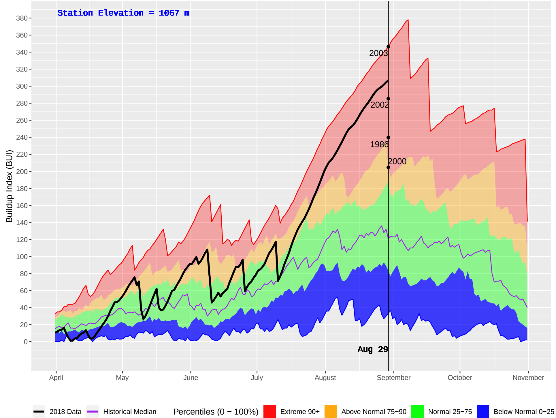
MCCUDDY (334) : Historical (1984–2016) and Current (2018) Daily Buildup Index (BUI)
