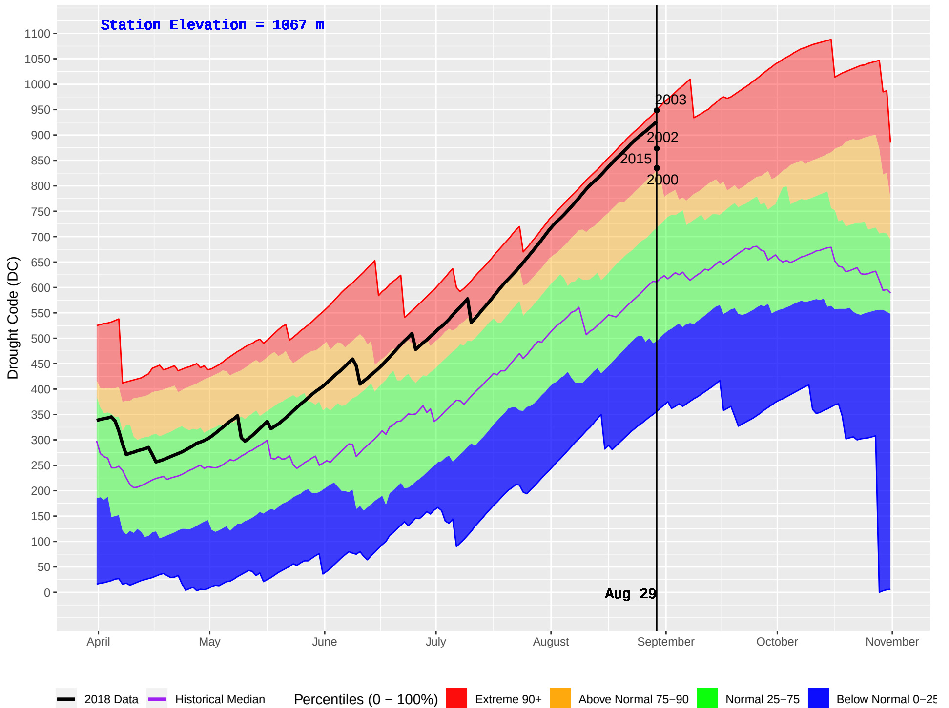
MCCUDDY (334) : Historical (1984–2016) and Current (2018) Daily Drought Code (DC)
