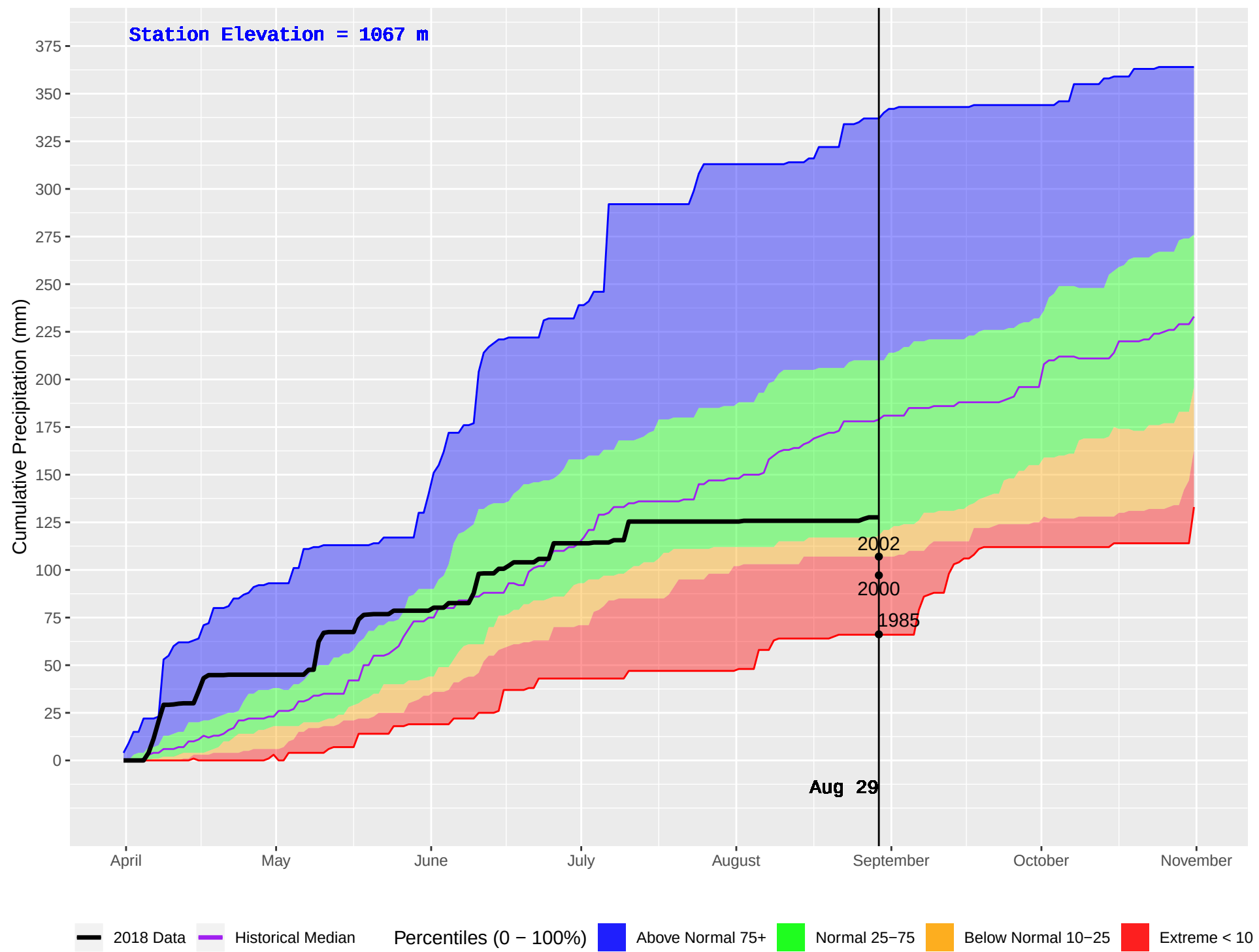
MCCUDDY (334) : Historical (1984–2016) and Current (2018) Daily Cumulative Precipitation
