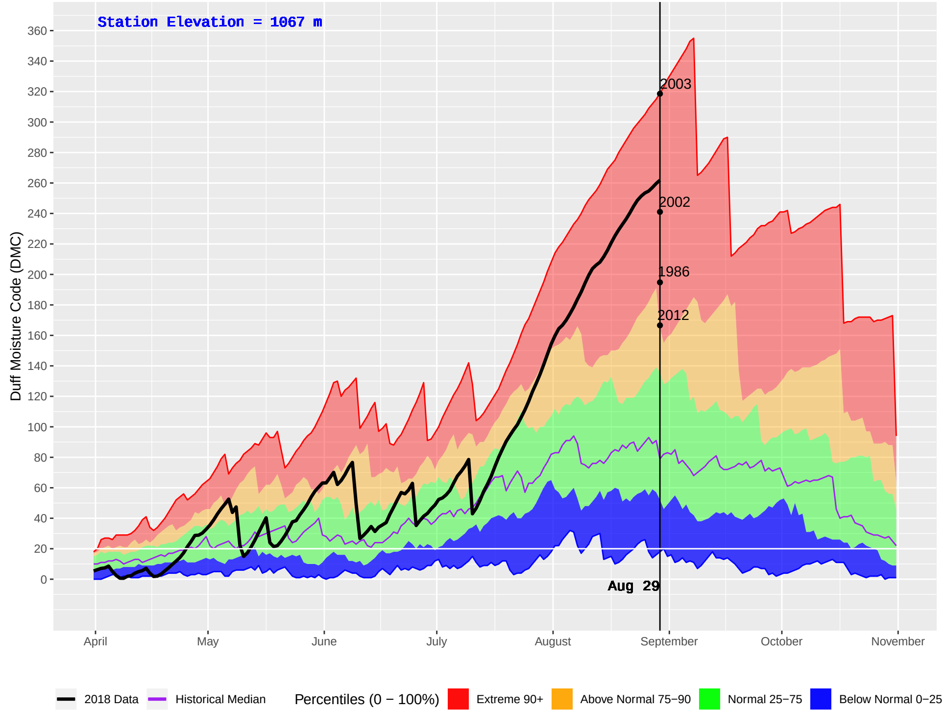
MCCUDDY (334) : Historical (1984–2016) and Current (2018) Daily Duff Moisture Code (DMC)
